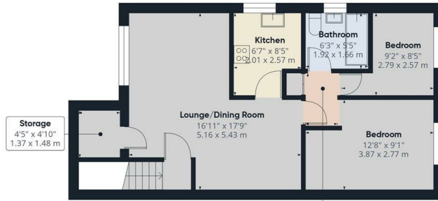
Inner Hall 3'2" x 5'7" 0.97 x 1.72 m
